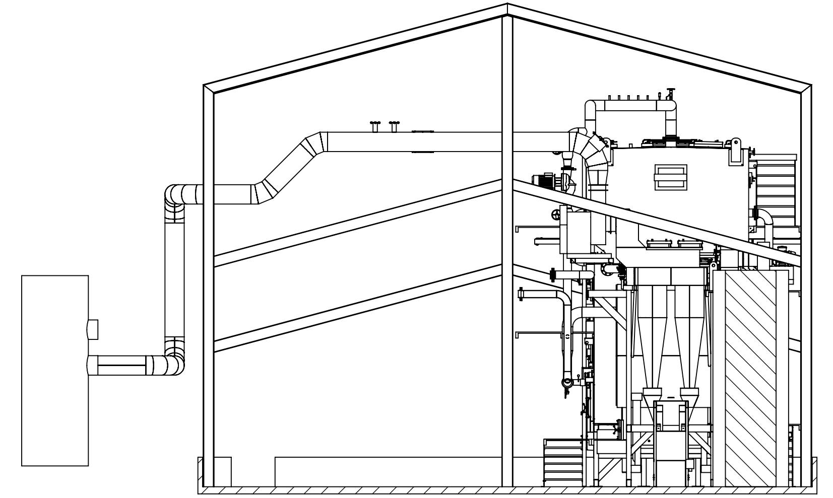
SECTION C-C
